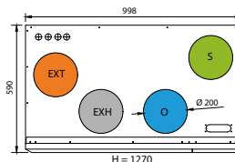
Dimension drawing right version
